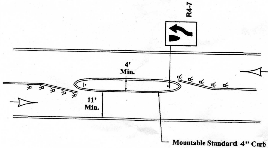
Figure A-7. RAISED MEDIAN ISLAND
